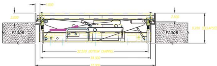
Typical pit installation
