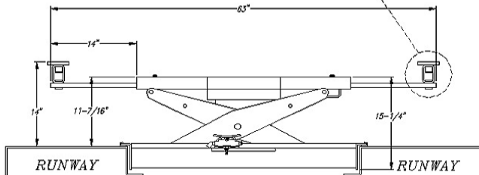
Jack Fully Raised with Arms extended
