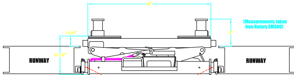
Wheel Assemblies (Adjustable: fits between 43"-57" between opening runways)
