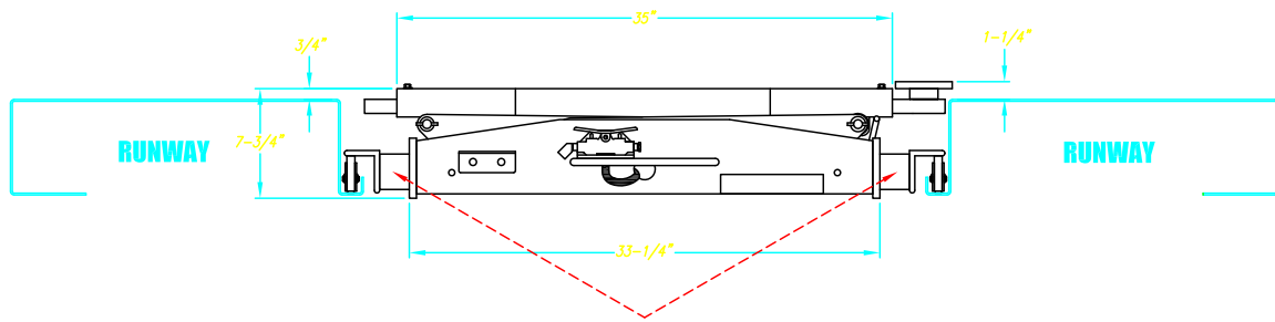
Wheel Assembly (Adjustable; Fits between 38"-52" between opening runways)
